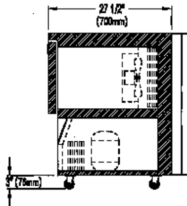
SIDE VIEW (SECTIONAL)
