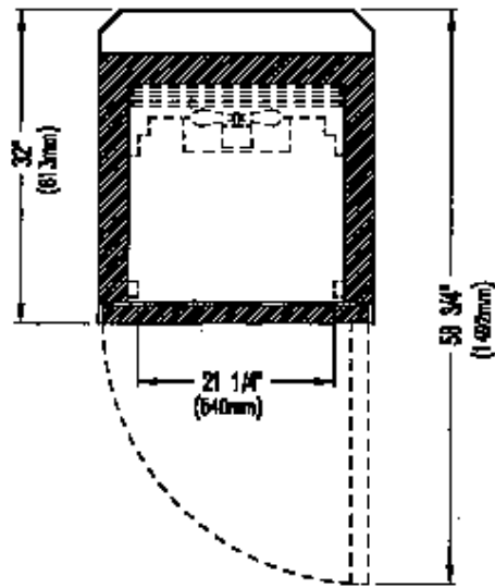
TOP VIEW (SECTIONAL)
